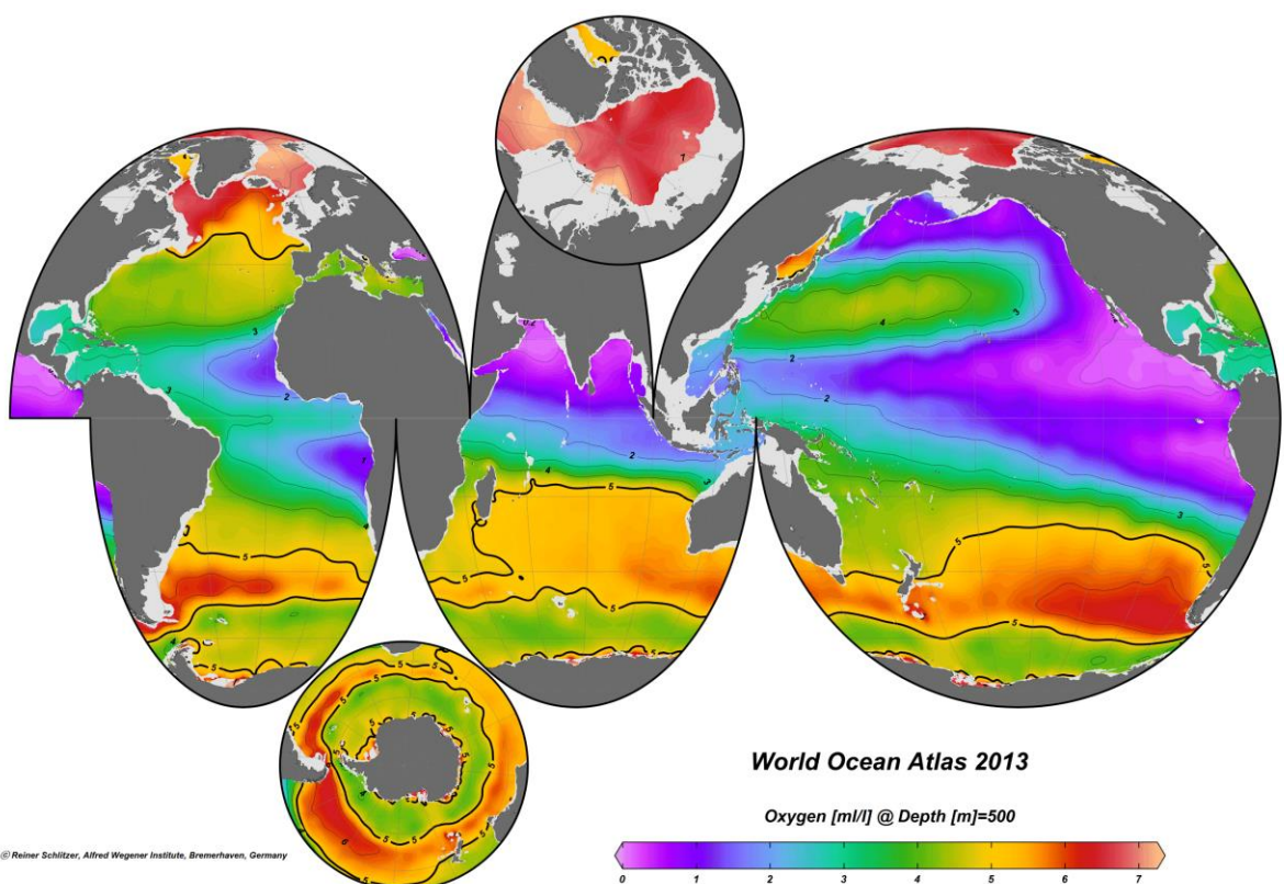
Figure 1-7: Oxygen distribution on the 500 m depth isosurface shown as interrupted map. Interrupted maps are produced via the "Save As Interrupted Map" option of the plot's context menu.
